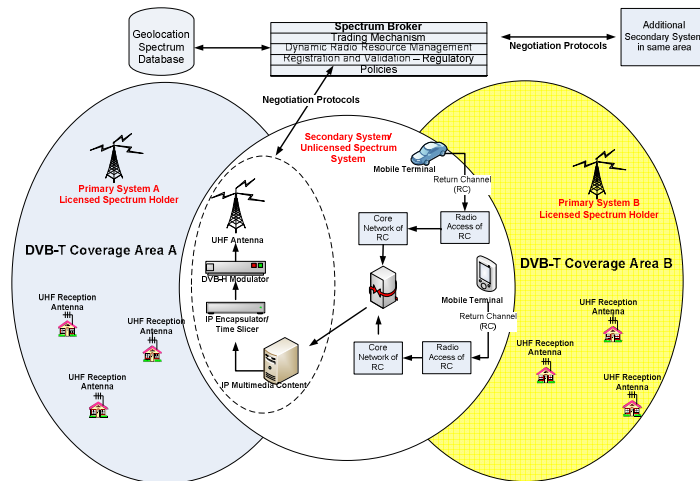
Figure 2 -Mobile TV network configuration in a cognitive radio approach
