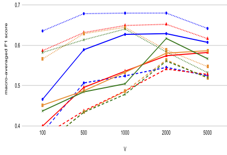
(a) BERT
