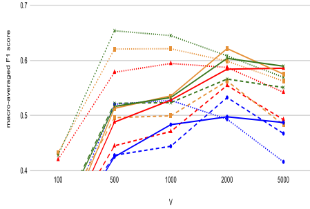
(c) GPT-2
