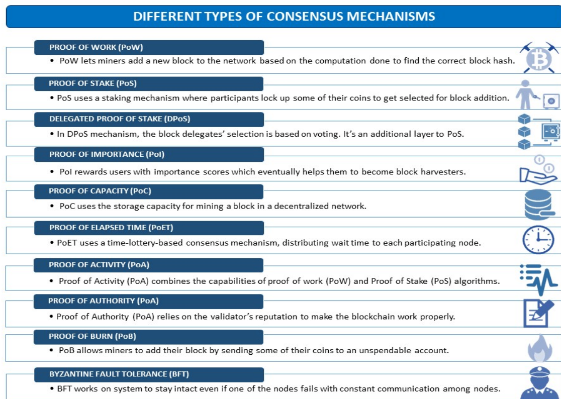
Figure 4: All Consensus mechanisms(Shiksha, 2023)
