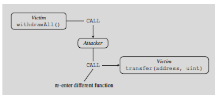
Figure 14: Call the Withdraw function instead of Deposit during the Re-entrancy Attack.
