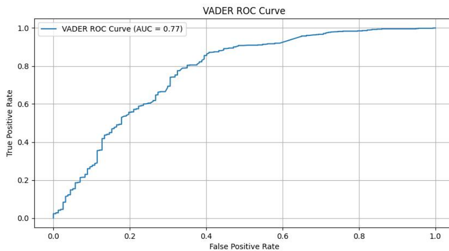
Figure 31: VADER ROC Curve
