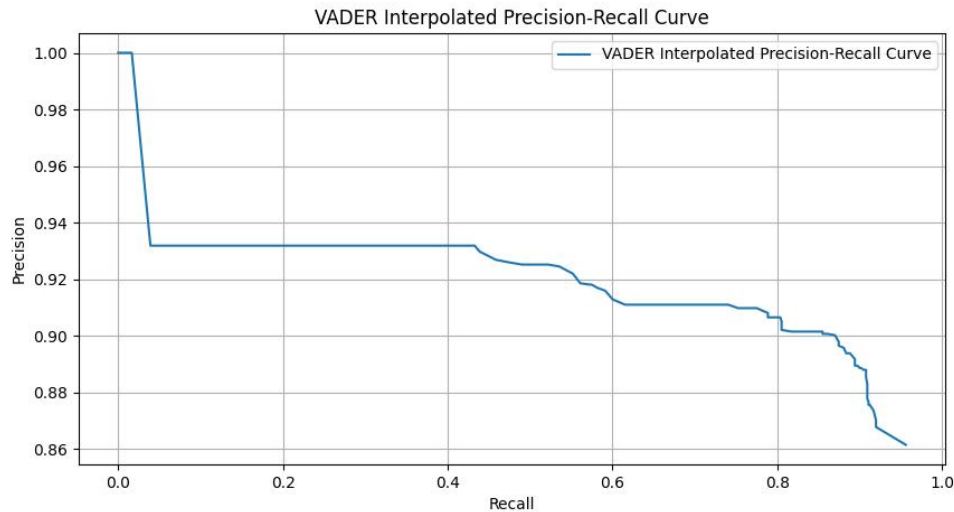
Figure 30: VADER Interpolated Precision-Recall Curve
