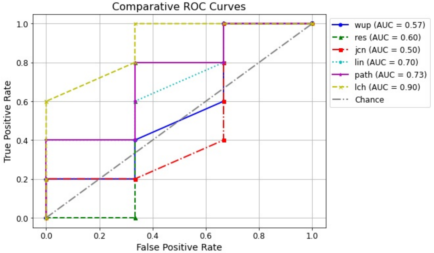
Figure 19: Comparative ROC Curves.
