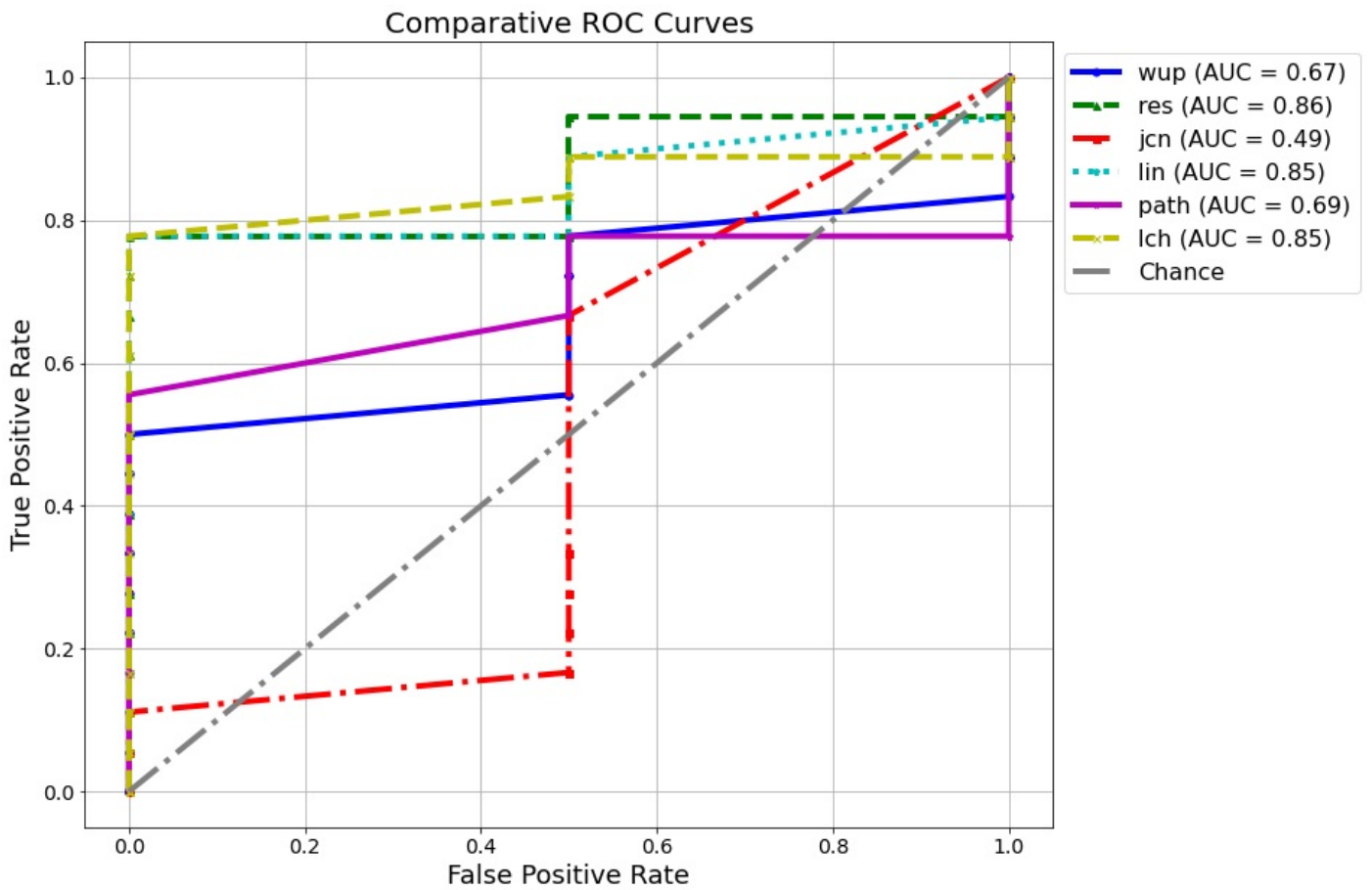
Figure 25: Comparative ROC Curves Diagram after the application of Advanced Algorithm on the the Amazon Dataset
