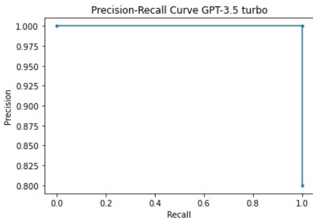
Figure 34: Precision-Recall Curve
